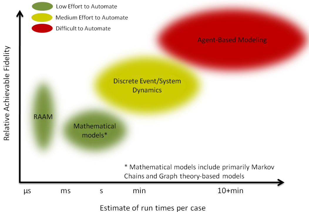
Figure 77: Fidelity vs Time per Case
