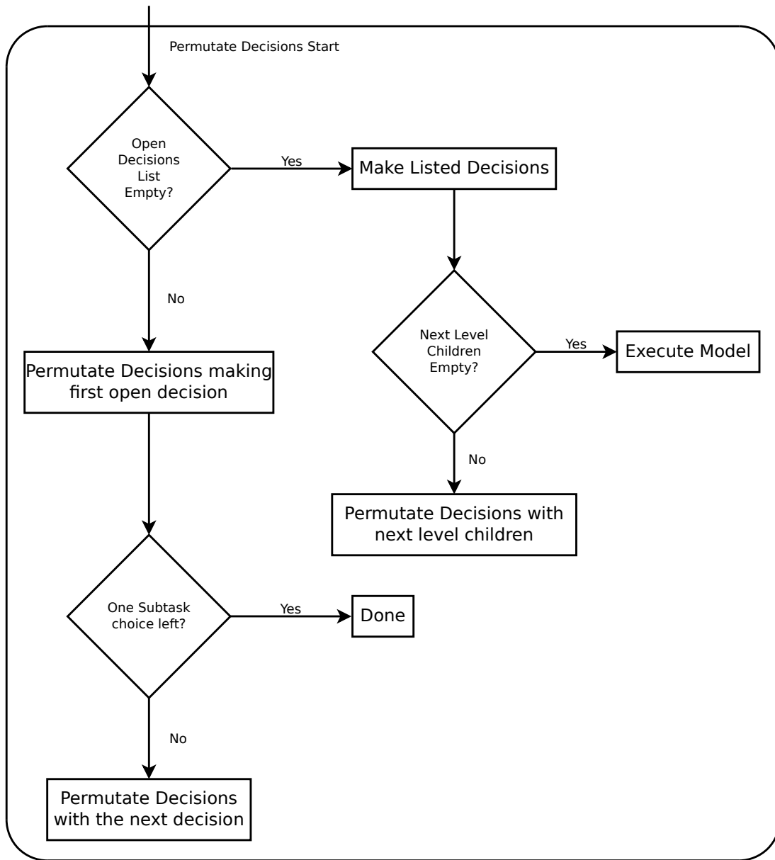
Figure 23: Permutate Decisions Flow Chart
